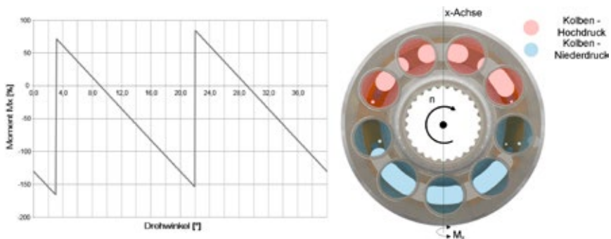
Abb. 5: Moment M_x
