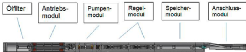
Abb. 1: MDA-Aggregat in Modulbauweise
